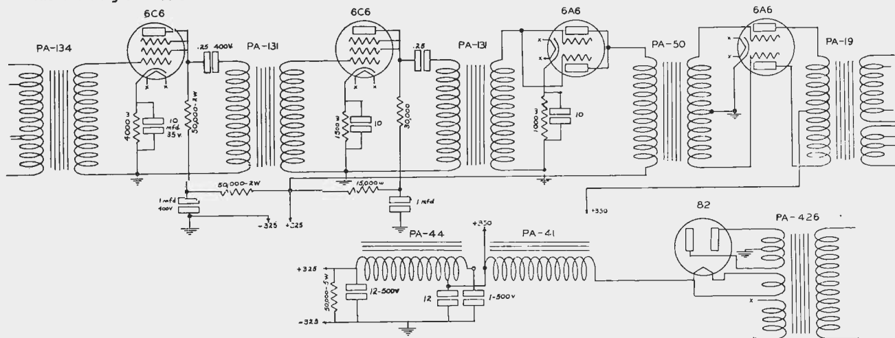
The 6A6 tube lends itself very well to PA work, particularly for mobile use. The amplifier shown will deliver 12 watts of audio. It can be either battery or A.C. operated. 6 Volt tubes are used throughout. The gain of approximately 100 DB makes this amplifier suitable for use with some of the new low level microphones and pickups.
