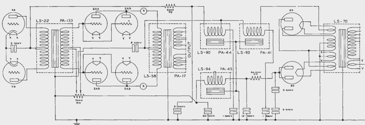
Push pull parallel 2A3 output power stage with fixed C bias and separate bias adjustment to balance plate current of output tubes. Shunt resonant rectifier filter used for highest filtering efficiency.
